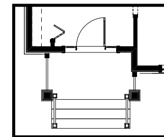
Front entry for Elevations B or C
