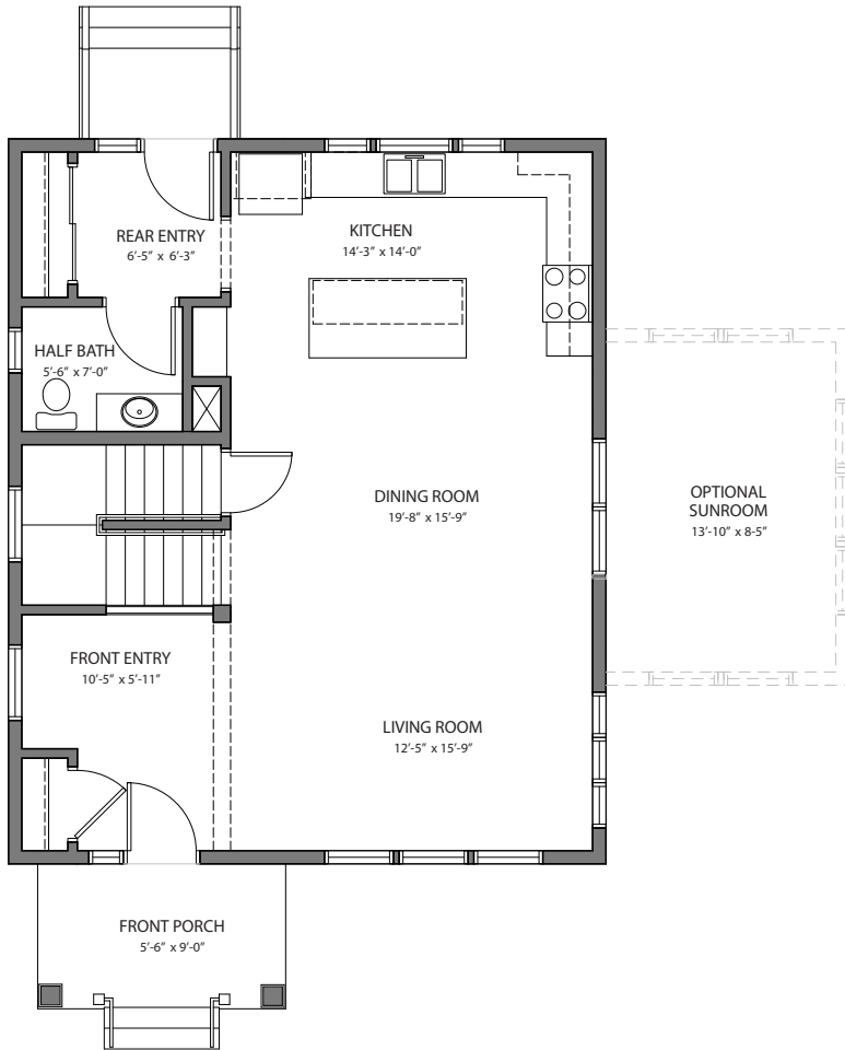
FIRST FLOOR
